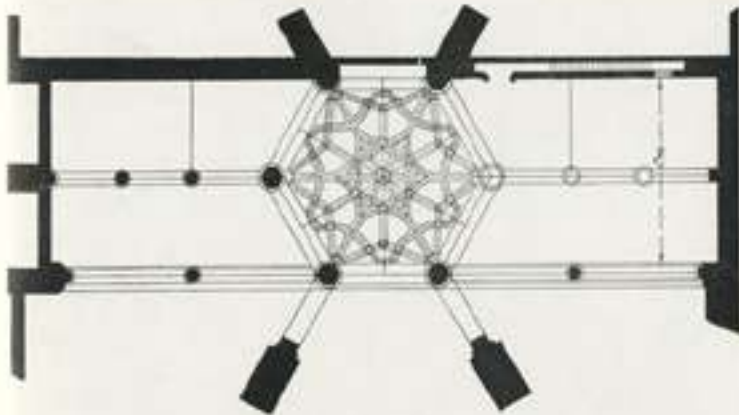
Plan and view of open chapel at Tepascalula, Oaxaca, 2nd half of 16th century Planta y vista de la capilla abierta de Tepascalula, Oaxaca, segunda mitad del siglo XVI
